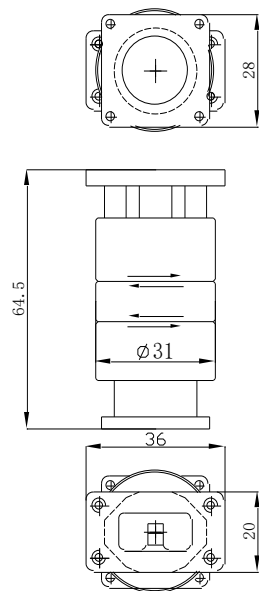
Ku Band I Type/circular waveguide Polarization Tracking Rotary Joint
