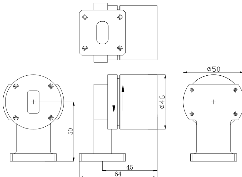
Ku Band L Type Waveguide Rotary Joint
