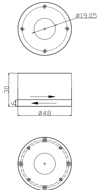
Ku Band Waveguide Rotary Joint II
