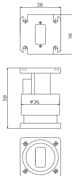
Ku Band Waveguide Rotary Joint I
