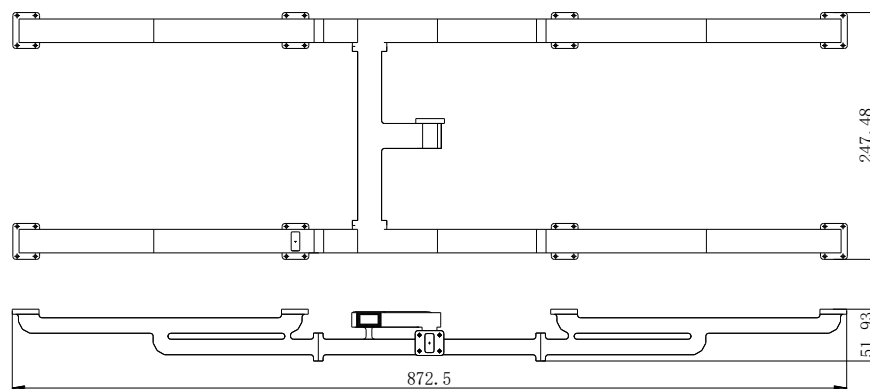
Ku Band Satellite Communication 8 in 1 Combiner
