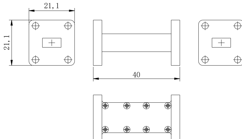
Ka Band Bandpass Filter
