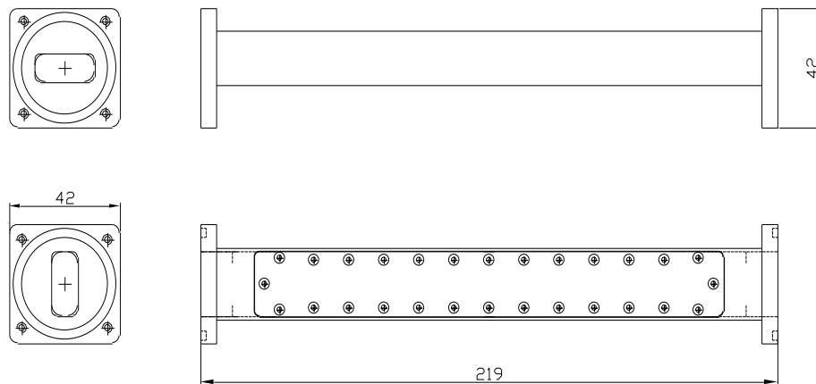
X Band High Altitude Waveguide Bandpass Filter
